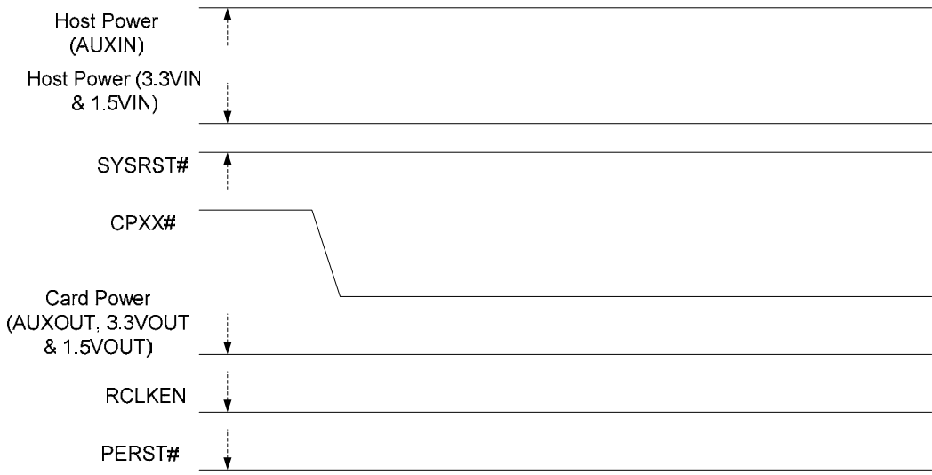
Fig.13 Host System In Standby Prior to Card Insertion
